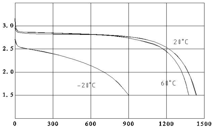
temperature characteristics(100mAh)
