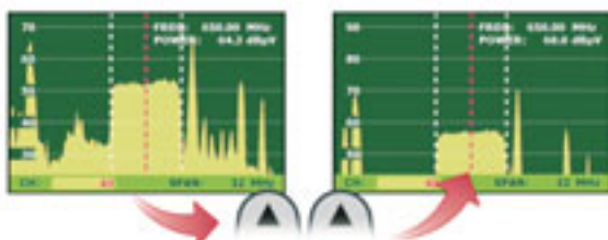
By pressing UP key twice the instrument sets the reference level from 70 to 90 dBµV.
