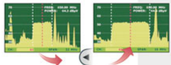
Starting from a SPAN of 32 MHz, we press LEFT key and we reduce view to 16 MHz.
