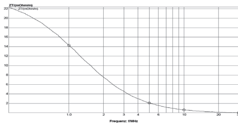
Kopplungswiderstand | Coupling resistance
